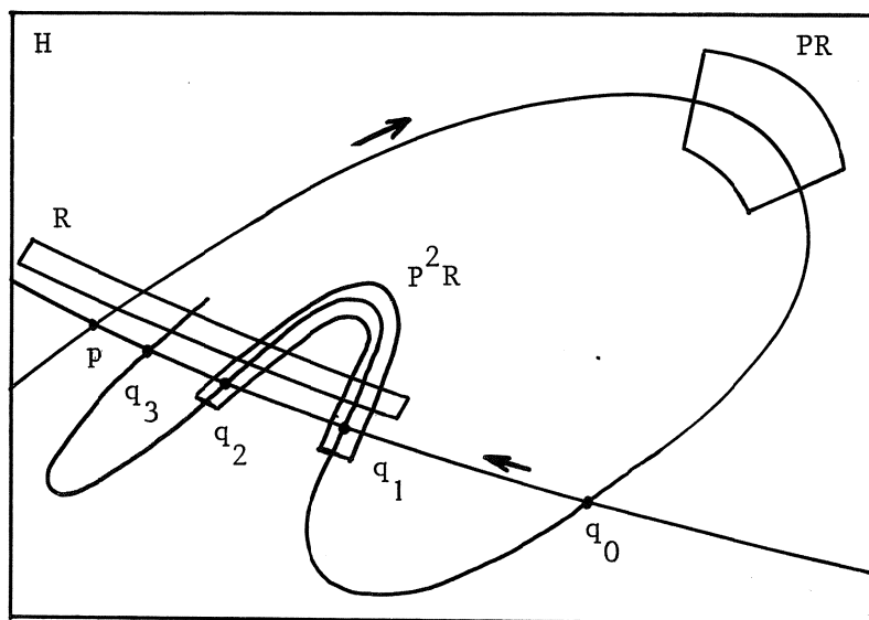
Fig. 6 The horse shoe mapping P^2
